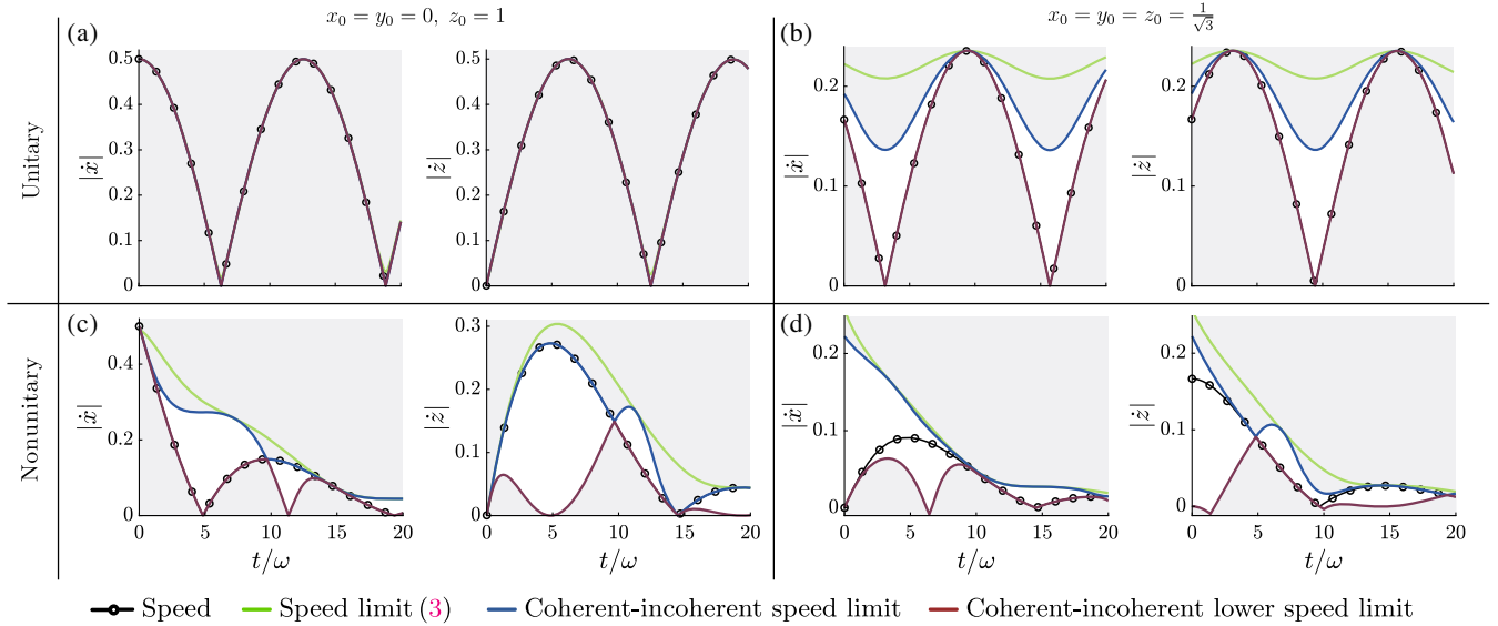
FIG. 1. Speed limits for observables on a qubit. The speed limit (3), derivable from the Cramér-Rao bound, and the coherent-incoherent speed limits (12) and (11) impose constraints on the rate \dot{a} at which observables evolve. We illustrate this on a qubit with a state parametrized by \rho = \frac{1}{2}(\mathbb{1} + x\sigma_x + y\sigma_y + z\sigma_z) and driven by the Hamiltonian H = (\omega/2)\sigma_y and dephasing along \sigma_z with a rate \kappa . Black lines with circles denote the speeds |\dot{x}| and |\dot{z}| of observables \sigma_x and \sigma_z , and blue (red) lines denote the coherent-incoherent (lower) speed limits. The gray areas denote rates forbidden by the coherent-incoherent speed limits. In green, the looser speed limit (3) appears inside the forbidden region. (a,c) The qubit is initialized in state z_0 = 1 and thus evolves in the y = 0 plane on and inside the Bloch sphere, which in turn implies that both observables \sigma_z and \sigma_x have coherent-incoherent decompositions that satisfy conditions for the saturation of Eq. (10), with \sigma_{\{z,x\}} = \alpha_C^{\{z,x\}}L_C + \alpha_I^{\{z,x\}}L_I . For unitary dynamics [ \kappa = 0 , (a)], this also means that the speed limit (3) saturates, and the three curves coincide. For open-system dynamics [ \kappa \neq 0 , (c)], the red and black curves coincide, but the speed limit (3) is looser except when \alpha_C^{\{z,x\}} = \alpha_I^{\{z,x\}} . Alternatively, whenever \alpha_C^{\{z,x\}} and \alpha_I^{\{z,x\}} have the same (different) sign, the coherent-incoherent (lower) speed limits saturate. (b,d) The coherent-incoherent speed limits (12) and (11) are not tight for a qubit initialized in x_0 = y_0 = z_0 = 1/\sqrt{3} , when the state does not evolve within the y = 0 plane, and the observables no longer have a decomposition solely in terms of L_C and L_I . Nevertheless, these bounds serve to constrain observables' dynamics more than the speed limit (3).
