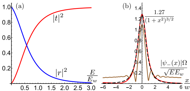
FIG. 2. (a) Transmission |t|^2 and reflection |r|^2 probabilities for the geometric scalar potential U(x) [Eq. (1)] as a function of the incoming energy E . (b) |\theta''\psi_D + 2\theta'\psi_D'|\sqrt{E_w/E} (red), its approximate form 1.27/(1+x^2)^{3/2} from Eq. (27) (black dashed), and |\psi_-(x)|\Omega/\sqrt{EE_w} (brown) for \Omega = 20E_w and E = E_w/50 . Excited state population can be determined via P_e \sim |\psi_-(0)|^2 \approx \frac{EE_w}{\Omega^2} , which agrees with Eq. (8), while the nonadiabaticity error is P_{\text{NA}} = \frac{k_y}{k} [|\psi_-(-L)|^2 + |\psi_-(L)|^2] \approx 9 \times 10^{-5} , which agrees with the approximate asymptotic formula [Eq. (29)] p_{\text{NA}} \approx 1.37\sqrt{E/E_w} e^{-1.75\sqrt{\Omega/E_w}} \approx 8 \times 10^{-5} .
