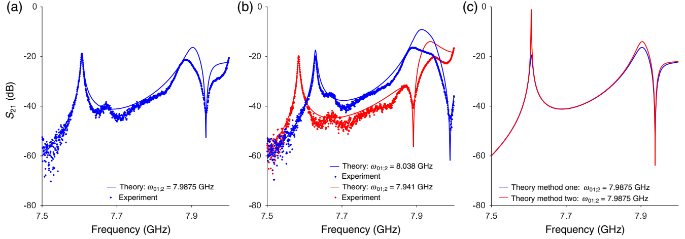
FIG. 6. Dependence of transmission S_{21} on drive frequency, dependence used for determining the coupling strength of the second qubit, i.e., the one at site N/2 + 1 = 9 . (a) Solid blue line is theoretical data for \omega_{01,2} = 7.9875 GHz while blue dots are experimental data. We choose parameters of the Hamiltonian such that the bound-state frequency, the transmission dip frequency, and the linewidth of the bound state match the experimental data. (b) Solid blue line is theoretical data for \omega_{01,2} = 7.941 GHz and blue dots are experimental data. Solid red line is theoretical data for \omega_{01,2} = 8.038 GHz and red dots are experimental data. (c) Comparison of transmission methods for \omega_{01,2} = 7.9875 GHz. The solid blue line is from method one, while the solid red line is from method two. The bound-state and transmission dip occur at the same frequencies for both methods.
