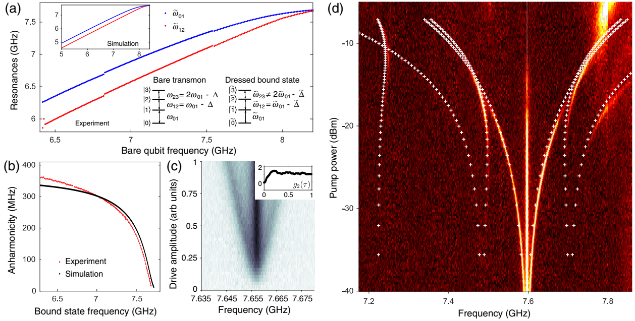
FIG. 2. Probing the bound-state energy levels. —(a) The anharmonicity of the bound state \tilde{\Delta} is dependent on bare transmon qubit frequency \omega_{01} , demonstrating a tunable on-site interaction strength. In blue (red), the first (second) transition of the bound state is measured across a range of bare qubit frequencies (inset: simulation). Upper left corner: level diagram of the bare transmon and dressed transmon. (b) Decreasing anharmonicity with increasing bound-state frequency shown in red for experimental data and black for simulation. (c) Power spectrum of a resonantly driven bound state for increasing drive amplitude. Sidebands are linearly displaced from the central peak with increasing drive amplitude, characteristic of the Mollow triplet. Inset: second-order autocorrelation measurement for drive amplitude = 0.2 is consistent with single photon, antibunched transport. (d) Emission spectrum of a resonantly driven ( \approx 7.59 GHz) bound state (induced by a qubit at 7.9 GHz, which is above the band edge located at 7.8 GHz) as a function of drive power. At low drive power, only the Mollow triplet is observed. With increasing power we see four additional sidebands, two on either side of the original Rabi sidebands, which together are the transitions between the three lowest levels of the anharmonic bound state ( |0\rangle , |1\rangle , |2\rangle ). The white crosses are from numerical simulations (see Appendix E). We have included five transmon qubit levels in our simulation. See text for the discussion of the seventh sideband around 7.25 GHz.
