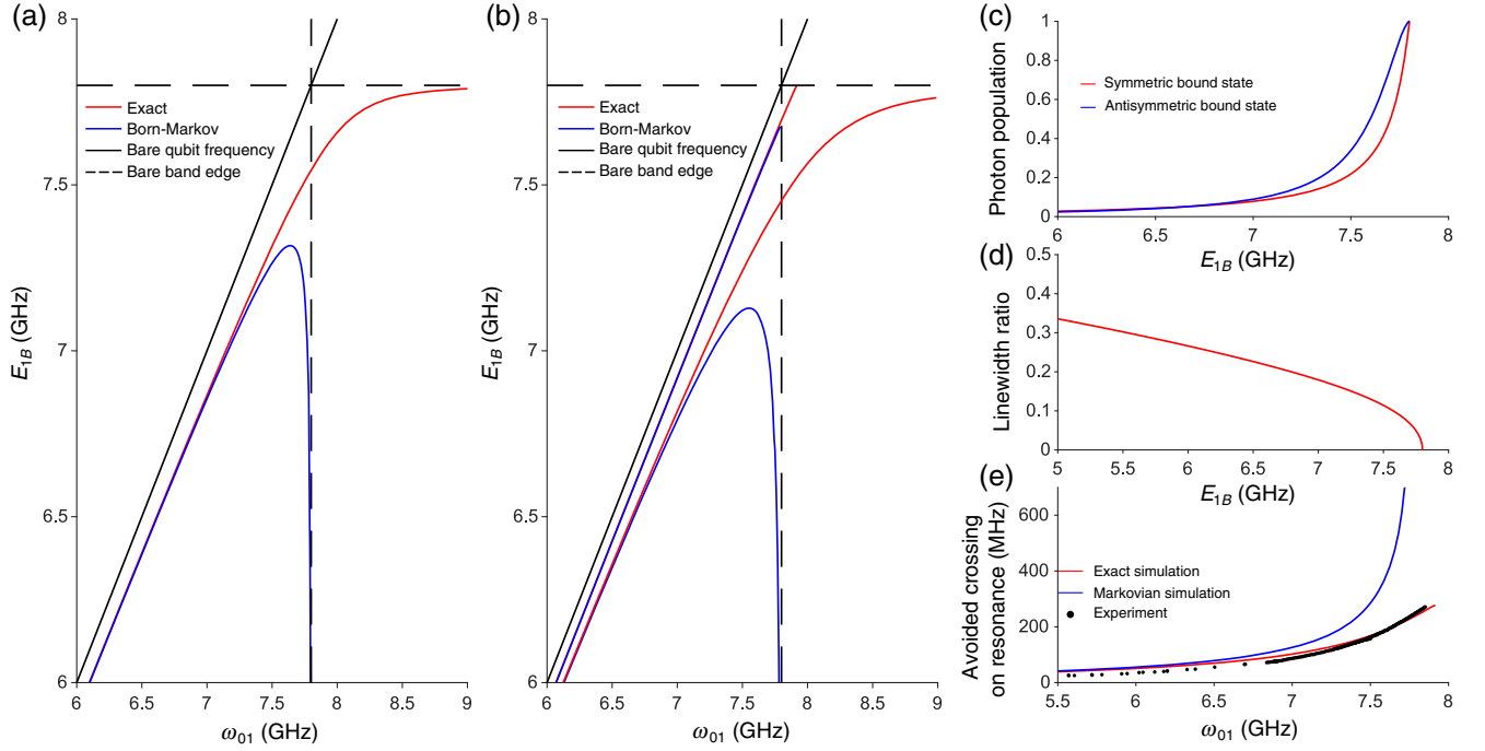
FIG. 8. Exact solution versus Born-Markov approximation. Here, the red lines are the exact solution while the blue lines are the Born-Markov approximation. The dashed black lines mark the band edge and the thick black line is the bare qubit frequency. Here, we take \omega_0 = 7.8 GHz, \alpha = 1.155 GHz, and g = 0.5275 GHz. (a) Single qubit. (b) Two qubits for |z_1 - z_2| = 1 . (c) Theoretical photon population of the bound states. (d) Linewidth ratio of the two bound states as a function of bound-state energy. (e) Avoided crossing on resonance versus bare qubit frequency. We see that the experimental data are well described by the Markovian solution only deep in the gap.
