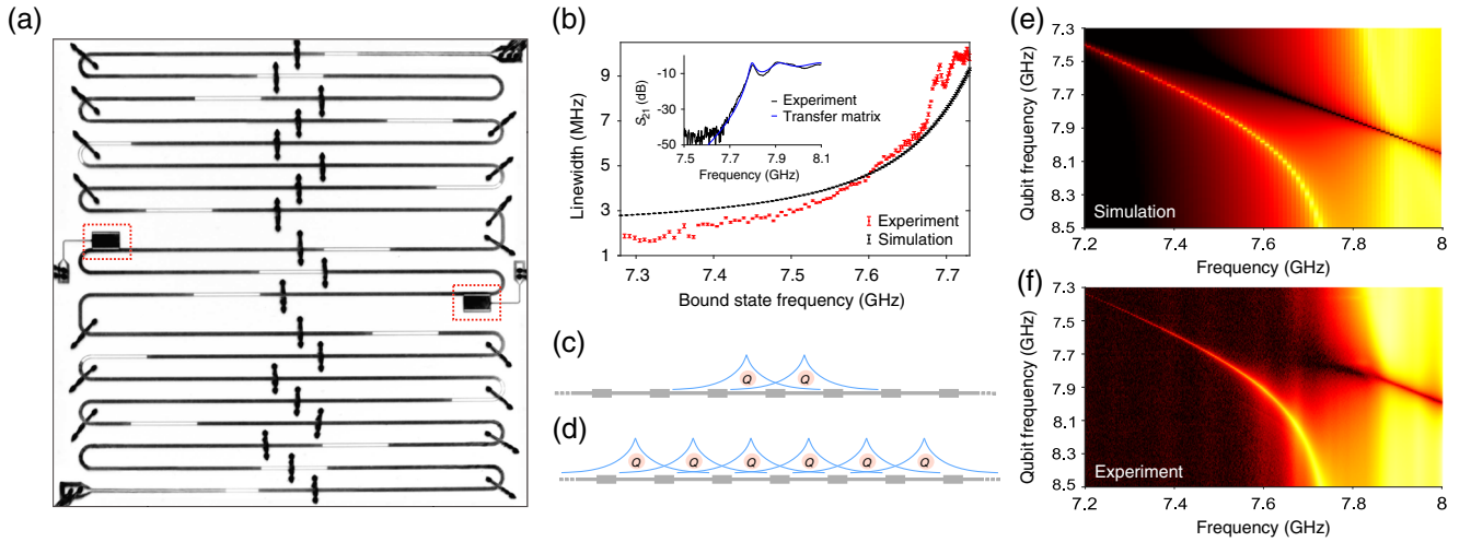
FIG. 1. A platform for interacting dressed bound states. —(a) A 16-site microwave photonic crystal is realized by alternating sections of high and low impedance coplanar waveguide. Two transmon qubits (multilevel, anharmonic energy ladder) are in neighboring unit cells in the middle of the device, centered in the high impedance sections for maximal coupling to the band edge at 7.8 GHz [all values presented in units of (2\pi) Hz, i.e., \omega_{BE} = 7.8 (2\pi) GHz]. For this experiment, the passband (band gap) refers to states above (below) the band-edge frequency. Each transmon is individually tunable in frequency via a local flux bias line. (b) Bound-state linewidth, an indirect measure of localization, varies with bare transmon qubit frequency. The wide range over which photon localization can be tuned indicates the feasibility of realizing a chain of strongly interacting bound states. Experimentally measured and simulated linewidths are shown in red and black, respectively. Inset: Overlay of simulated S_{21} from the transfer matrix method (blue) and measured high-power S_{21} (black) shows good agreement in bare crystal characteristics. (c) The interaction between bound states will be determined by overlap of their localized photonic envelopes with the qubits. (d) One can couple more qubits to the band edge by adding them to other cells of the photonic crystal. In such a system, the localization-length-dependent interaction of the bound states would preserve the spatial organization of qubits across the crystal, and determine the many-body structure of the interactions. (e) Experimental data and (f) hopping model simulation for S_{21} vs single-qubit frequency and probe frequency. The bare band edge is at 7.797 GHz. The bright peak in the band gap is the dressed qubit-photon bound state. The bound state always exists within the band gap for qubit frequencies (the other qubit is far detuned and has negligible effect) both above and below the band edge—a clear signature of non-Markovianity.
