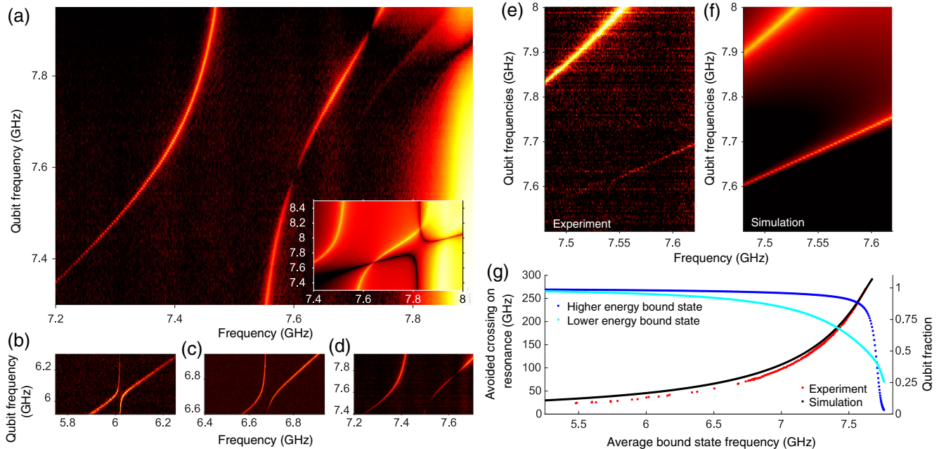
FIG. 3. Interacting bound states. —Interaction between bound states is characterized by the avoided crossing (observed in S_{21} measurement) that arises while tuning one qubit ( y axis) through resonance with the other (fixed). (a) An avoided crossing of 240 MHz is observed when the fixed qubit is at 7.73 GHz. The two points where transmission amplitude of a bound state dims are understood as the bound-state peak being resonant with the qubit frequency. (a), inset—Hopping model simulation of the one-excitation manifold is consistent with experimental observation. The Lamb shift in the hopping model originates from next-nearest-neighbor interaction between coupled cavities. (b),(c),(d) Tunable bound-state interaction strength is illustrated in example bound-state avoided level crossings for a fixed qubit whose bare frequency is circa 6.125, 6.75, and 7.625 GHz. As qubits are detuned further from the band edge, bound states are more tightly localized, reducing overlap and thus reducing interaction. (e),(f) Transmission when the qubits are on resonance across a range of qubit frequencies in the experiment and the simulation, respectively. The uneven linewidths of the two bound states when they occur at the same frequency suggest they are symmetric (higher-frequency bound state) and antisymmetric (lower-frequency bound state) states (see main text). (g) Bound-state avoided crossing and qubit population (from simulation) as a function of average bound-state frequency. A steady reduction in interaction strength occurs with increasing detuning from the band edge (moving deeper into the band gap) due to increasing localization of the bound states. Hopping model simulation (black) captures this detuning-dependent behavior observed in experiment (red). Near the band edge, both bound states (blue and cyan) have a significant photonic contribution.
