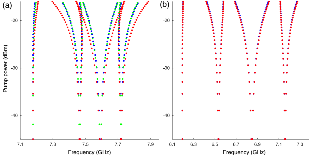
FIG. 9. Theoretical simulations of the emission spectrum for different pump powers. Here, the blue squares are numerical results obtained from the total Hamiltonian Eq. (E1), the green squares are from the dressed-transmon Hamiltonian Eq. (E2), and the red squares are from Eq. (E2) but with \cos \theta = 1 . (a) Here, \omega_{01} = 7.97 GHz, and the bound-state frequency is 7.591 GHz. Using the appropriately reduced matrix element ( \cos \theta < 1 , blue squares) is crucial in obtaining accurate results using Eq. (E2). (b) Here, the bare qubit frequency of 7 GHz and the bound-state frequency of 6.847 GHz are both far from the band edge, so that \cos \theta \approx 1 and the reduction in the matrix element can be neglected, so all three data sets lie on top of each other.
