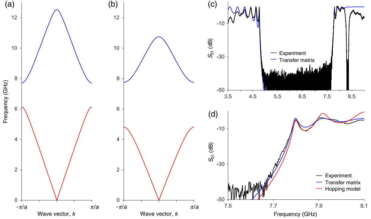
FIG. 5. First two bands of simulated dispersion for Z_{lo} = 25 \Omega , Z_{hi} = 124 \Omega and (a) L_{lo} = 0.45 mm, L_{hi} = 8 mm (parameters from [13]), and (b) L_{lo} = 1.2 mm, L_{hi} = 7.8 mm (parameters from present paper). (c) Overlay of simulated S_{21} from the transfer matrix method [blue; same parameters as (b)] and measured high-power S_{21} (black) shows good agreement in bare crystal characteristics. (d) Overlay of simulated S_{21} from the transfer matrix method [blue; same parameters as (b)] and from the hopping model [red; with \kappa = 1 GHz and \kappa_0 = 4 MHz] and measured high-power S_{21} (black) near the band edge. Drop in transmission circa 8.3 GHz is due to TWPA dispersion, not device defect.
