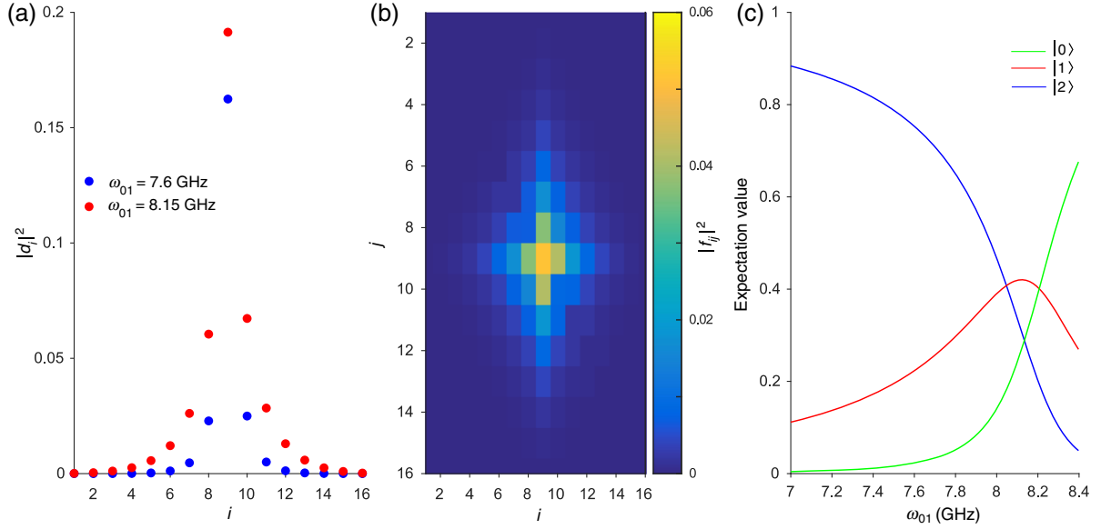
FIG. 10. Visualizing the two-photon bound state. Here, the transmon qubit is on site nine. (a) The blue dots are |d_i|^2 versus position for \omega_{01} = 7.6 GHz. The red dots are |d_i|^2 for \omega_{01} = 8.15 GHz as a function of position. (b) Plot of |f_{i,j}|^2 as a function of i and j for \omega_{01} = 8.15 GHz. (c) The population of transmon qubit levels in the two-excitation ground state of H_{\text{tot}} as a function of bare qubit frequency.
