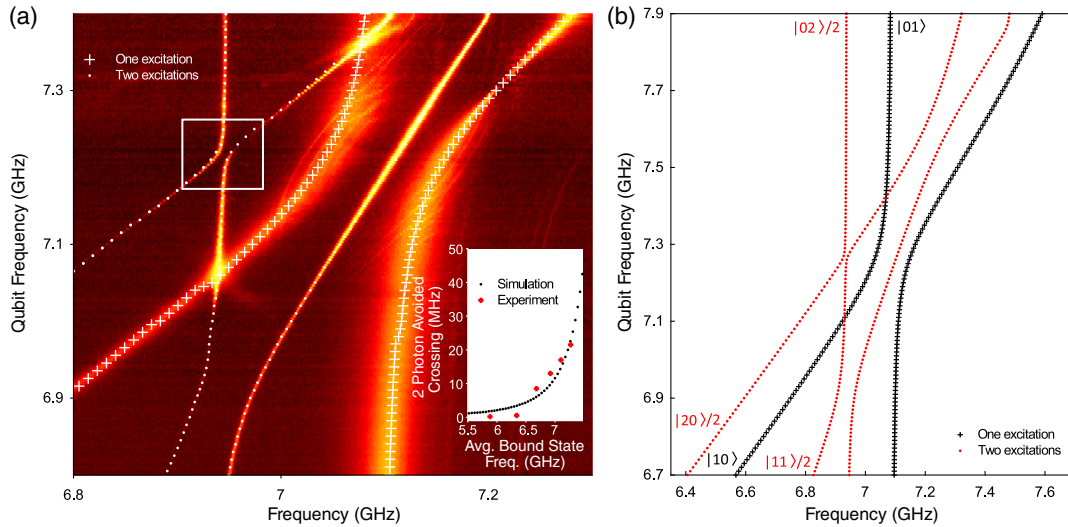
FIG. 4. Interaction between two-excitation levels of two bound states. —(a) Spectroscopic measurement while tuning one bound state through the other (qubit fixed at 7.2 GHz), reveals survival of strong interaction into the two-excitation manifold. Crossed and dotted lines are guides to the eye to discern the levels belonging to the first ( |01\rangle and |10\rangle ) and second ( |02\rangle , |20\rangle , and |11\rangle ) excitation manifolds, respectively. Here, we have labeled our states as |\text{transmon one}, \text{transmon two}\rangle . In addition to the |02\rangle(|20\rangle) and |11\rangle avoided level crossing, we also detect a two-photon virtual interaction between |02\rangle and |20\rangle (white box). This interaction—fourth order in coupling g —manifests itself in avoided level crossings up to and exceeding 20 MHz. For comparison, the |02\rangle(|20\rangle) - |11\rangle and |01\rangle - |10\rangle interactions are second order in g and thus both are significantly stronger. Inset: two-photon avoided crossing strength versus average bound-state frequency. (b) Numerical simulation for fixed bare qubit frequency of 7.27 GHz, with the one (two) excitation manifold in black (red).
