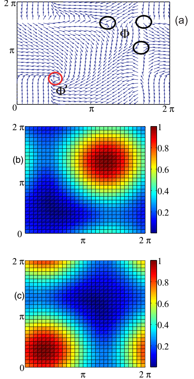
Fig. 3: (Colour on-line) (a) \Omega(\theta_1, \theta_2) for fixed \Phi and \Phi' . \theta_1 and \theta_2 changes from zero to 2\pi . This plot has been produced for 4 atoms in the hard-core limit on a 5 \times 5 lattice ( \alpha = 0.32 ). (b) and (c) surface plots of \det\Lambda_\Phi and \det\Lambda'_\Phi (blue is lower than red). \theta_1 and \theta_2 changes from zero to 2\pi . The total vorticity corresponding to each of the trial function ( \Phi or \Phi' ) indicates a Chern number equal to one for the two-dimensional ground-state manifold.
