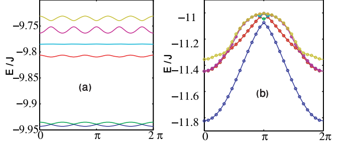
Fig. 2: (Colour on-line) Low-lying energy levels as a function of twist angles. For finite \alpha the ground-state energy oscillates as a function of twist angles and for high \alpha \gtrsim 0.4 the oscillations reach the excited levels. Panel (a) shows lowest-energy levels for \alpha = 0.32 (4 atoms on a 5 \times 5 lattice) while (b) shows the five lowest-energy levels for \alpha = 0.4 (5 atoms on a 5 \times 5 lattice). In both plots, \theta_2 = \pi and \theta_1 is varied from zero to 2\pi .
