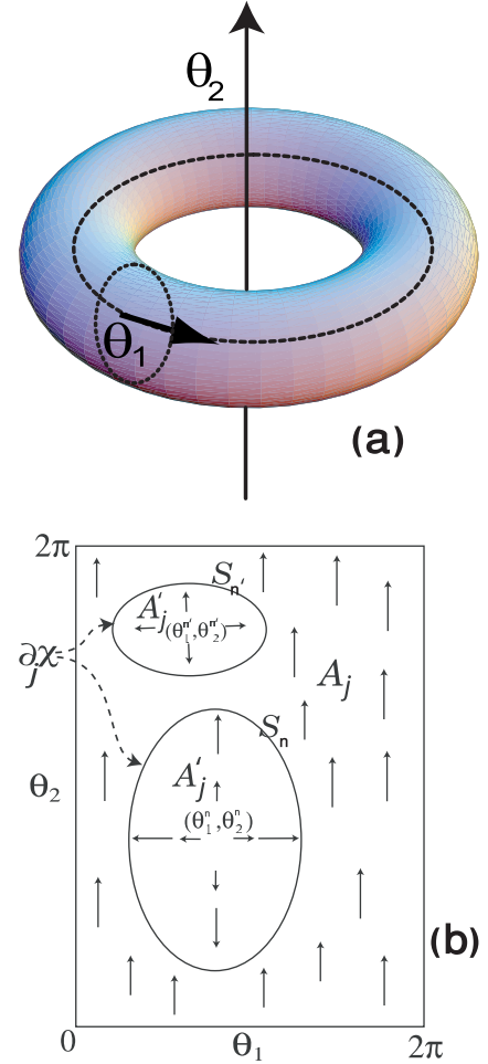
Fig. 1: (Colour on-line) (a) Twist angles of the boundary condition as the result of two magnetic fluxes threaded the torus. (b) Redefining the vector potential around the singularities: A_j is not well-defined everywhere on the torus of the boundary condition. Therefore, another vector field \mathcal{A}'_j with different definition should be introduced around each singularity (\theta_1^n, \theta_2^n) of A_j . However, A_j and \mathcal{A}'_j are related to each other with a gauge transformation \chi and the Chern number depends only on the loop integrals of \chi around those singularity regions.
