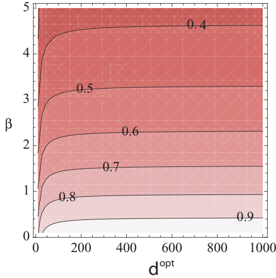
FIG. 3. (Color online) For large optical densities, the transmission on resonance ( \delta = \delta_0 ) only depends on \beta = d^{\text{opt}}(\frac{\Gamma}{\Delta_1})^2 .
