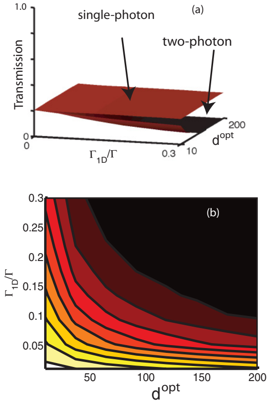
FIG. 20. (Color online) (a) One-photon state is partially transmitted ( T_1 ) while the two-photon state transmission ( T_2 ) is suppressed due to the nonlinear absorption. This suppression is more pronounced for higher optical density and cooperativity. (b) Correlation function g_2(\tau = 0) of the transmitted light when the frequency is set to the single-photon transmission resonance with T \simeq 20\% and \frac{\Delta_2}{\Gamma} = 0 .
