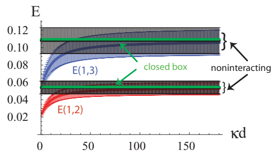
FIG. 9. (Color online) Energy of two-photon states. By increasing the interaction strength ( \kappa d \gg 1 ) the energy of interacting particles [red, E(1,2) ; blue, E(1,3) ] reaches that of the noninteracting particles (black). For a large system (in this case d = 30 \gg 1 ), the energy limit is equal to energy of particles in a closed box (green). The error bars show that imaginary part of the energies.
