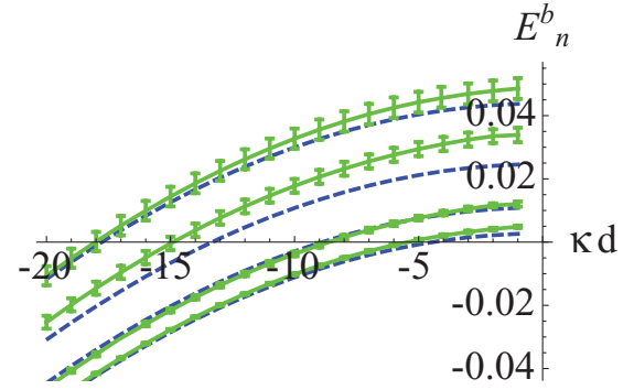
FIG. 12. (Color online) Energy of bound states versus strength of nonlinearity. Green (solid) curves are obtained by solving transcendental Eqs. (71). Blue (dashed) curve are estimated based on E_n^b \simeq (\frac{n\pi}{d})^2 - \frac{\kappa^2}{2} . In this plot, d = 30 .
