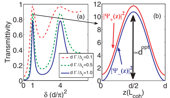
FIG. 2. (Color online) Linear case. (a) Transmittivity as a function of two-photon detuning. Transmission peaks are attenuated because of linear loss on |a\rangle \rightarrow |b\rangle transition which is plotted for three different loss rates \beta = d\Gamma/\Delta_1 . (b) When the system is tuned on a transmission resonance ( \sqrt{\delta_0} d = n\pi ), the field inside the medium is amplified.
