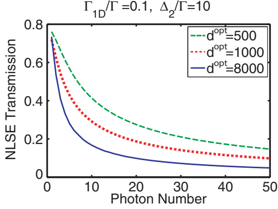
FIG. 6. (Color online) Transmission vs the number of incident photons. For each d^{\text{opt}} , \Gamma/\Delta_1 is chosen so that the system exhibit a similar transmission for one photon.
