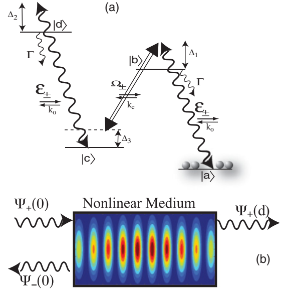
FIG. 1. (Color online) (a) Four-level atomic system for creating strong nonlinearity. Counterpropagating control fields modulate the EIT for the forward- and backward-propagating probe, and the |c\rangle \rightarrow |d\rangle transition gives rise to a Kerr-type nonlinearity. (b) The light is confined in the transverse direction due to the presence of the waveguide and experiences an effective Bragg grating due to the presence of the counterpropagating light.
