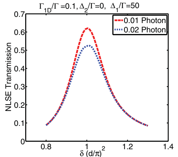
FIG. 7. (Color online) Due to nonlinear absorption, the transmission is suppressed for higher intensities. The integrated intensities inside the system are related to the number of present field quanta. The optical depth for these calculations is chosen to be d^{\text{opt}} = 3000 .
