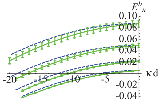
FIG. 10. (Color online) Energy of bound states versus strength of nonlinearity. Green (solid) curves are obtained by solving transcendental Eqs. (71). Blue (dashed) curves are estimated based on E_n^b \simeq 2(\frac{n\pi}{d})^2 - \frac{\kappa^2}{2} . In this plot d = 30 .
