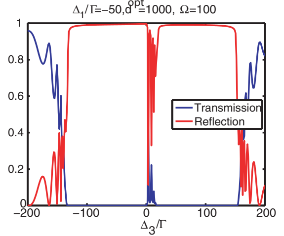
FIG. 24. (Color online) Band-gap structure for strong control fields ( \Omega > \Delta_1 ).
