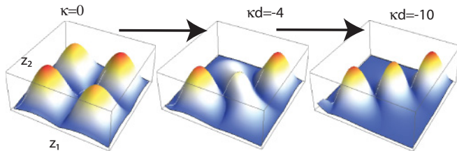
FIG. 11. (Color online) The amplitude of the two-photon wave function for a bound state when the system is not driven. By increasing interaction, photons becomes more bunched. (k_1, k_2) \simeq (\frac{n\pi}{d}) \pm i\frac{\kappa}{2} . For this plot, d = 60; n = 3 .
