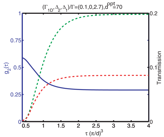
FIG. 19. (Color online) g_2(\tau = 0) reaches the steady-state after a time interval which is set by the bandwidth of the system, one-photon state (green dotted line) is partially transmitted while the two-photon state (red dashed line) is strongly attenuated due to the nonlinear absorption. This plot has been generated for a system with \Gamma_{1D}/\Gamma = 10\% and d^{\text{opt}} = 70 .
