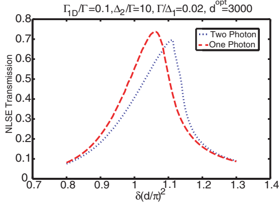
FIG. 4. (Color online) Due to nonlinearity, in the perturbative limit, the transmission spectrum shifts for different intensities. The integrated intensities inside the system are related to the number of present field quanta. The optical depth for these calculations is chosen to be d^{\text{opt}} = 3000 .
