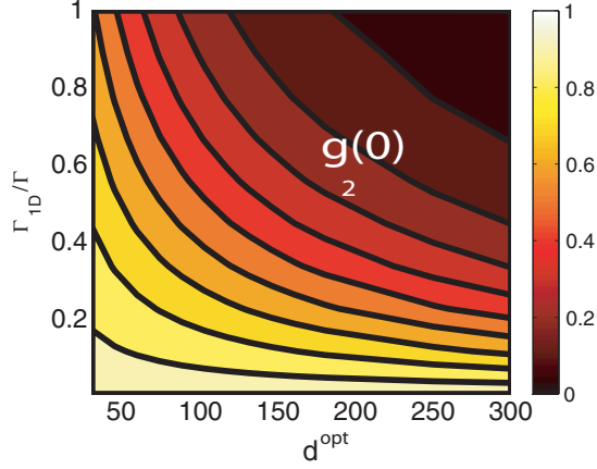
FIG. 17. (Color online) Repulsive photons. Correlation function g_2(\tau = 0) of the transmitted light when the frequency is set to the single-photon transmission resonance with T_1 \simeq 20\% and \frac{\Delta_2}{\Gamma} = 5 .
