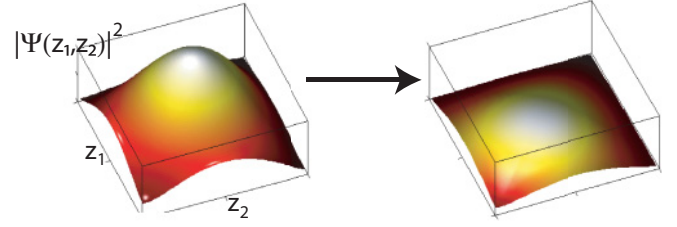
FIG. 21. (Color online) In the presence of the nonlinear absorption ( \frac{\Delta_2}{\Gamma} = 0 ), the two-photon wave function is strongly suppressed comparing to the absence of the nonlinear absorption ( \Delta_2 \gg \Gamma ). These plots has been generated for a system with \Gamma_{1D}/\Gamma = 10\% , T_1 \simeq 20\% , and d^{\text{opt}} = 70 .
