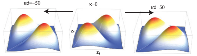
FIG. 8. (Color online) The amplitude of the two-photon wave function for (m = 1, n = 2) mode when the system is not driven. By increasing the interaction, photons self-organize inside the medium and exhibit antibunching (depletion of diagonal elements). For this plot, d = 30 .
