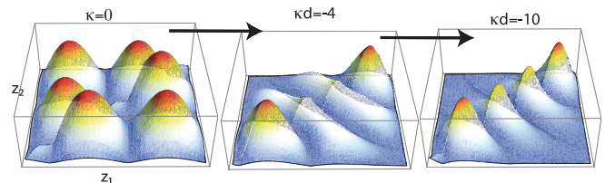
FIG. 13. (Color online) The amplitude of the two-photon wave function for a bound state for a nondriven system. By increasing interaction, photons becomes more bunched. (k_1, k_2) \simeq (\frac{n\pi}{\sqrt{2}d}) \pm i\frac{\kappa}{2} . For this plot, d = 60; n = 3 .
