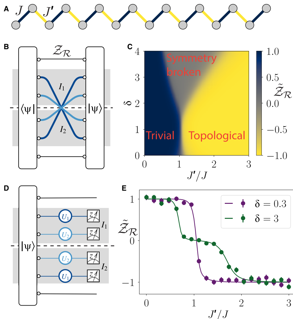
Fig. 1. Measuring the MBTI \tilde{\mathcal{Z}}_{\mathcal{R}} for the extended bosonic SSH model. (A) Schematic illustration of the model Eq. 1, where the nearest-neighbor spin-exchange coefficients alternate between the bonds. (B) The partial reflection invariant \mathcal{Z}_{\mathcal{R}} (Eq. 2) is defined as the expectation value of a partial reflection operator \mathcal{R}_I (visualized by the blue lines) for the many-body state |\psi\rangle . The dashed line between the intervals I_1 and I_2 indicates the reflection center. (C) In terms of the normalized invariant \tilde{\mathcal{Z}}_{\mathcal{R}} , the full-phase diagram of the extended bosonic SSH model is revealed here for a system size of N = 48 spins and n = 6 reflected pairs of spins. We find three phases with different quantized values of \tilde{\mathcal{Z}}_{\mathcal{R}} . (D) Protocol to measure \tilde{\mathcal{Z}}_{\mathcal{R}} via statistical correlations between randomized measurements, implemented with local random unitaries applied symmetrically around the central bond. (E) The results of simulated experiments allow us to identify topological phase transitions. The solid lines are results from DMRG, whereas the dots with error bars represent estimations from simulated randomized measurements with N_U = 512 unitaries and N_M = 256 measurements per unitary.
